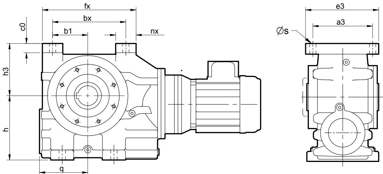
STANDARD UNIT WITH TOP MOUNTED FEET
